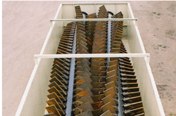
SPIRAL PADDLES FOR CONTINUOUS AGITATION
