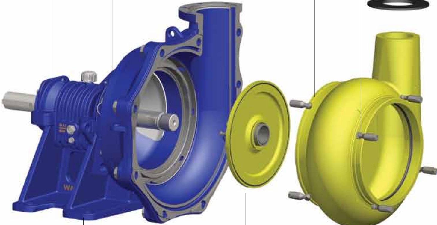
Interchangeable metal liners and impeller
